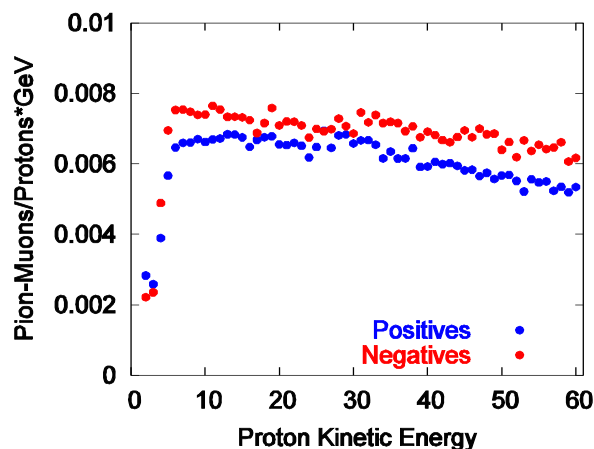
Figure 3: Muon production efficiency for a mercury-jet target as a function of proton driver beam energy.
