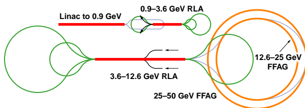
Figure 5: Neutrino Factory muon acceleration scheme
