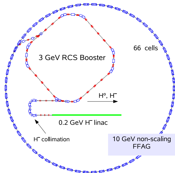
Figure 2: 10 GeV proton driver based on a synchrotron booster and an FFAG accelerator
