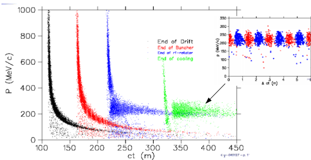
Figure 4: Simulation of muon front-end with adiabatic bunching scheme
