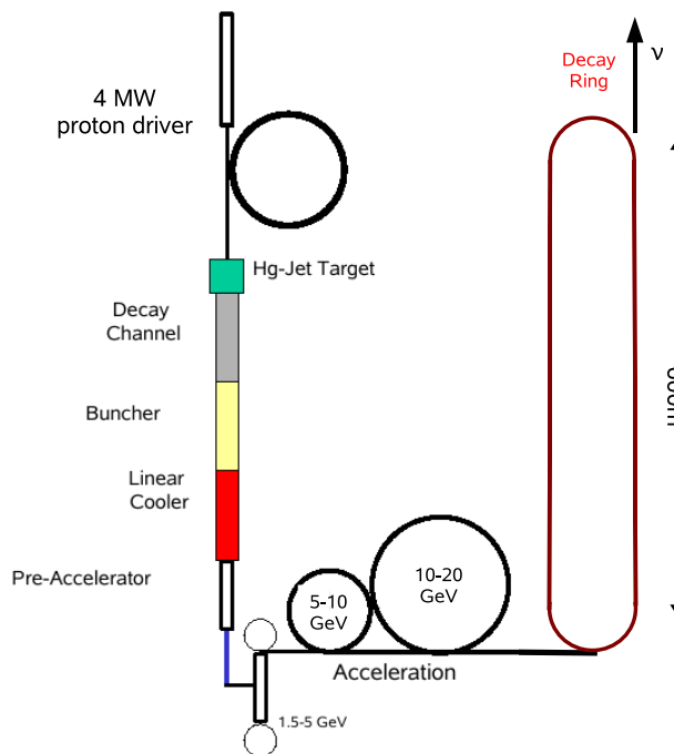
Figure 1: Schematic layout of a neutrino factory
