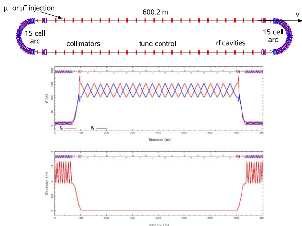
Figure 6: Racetrack decay ring; betatron and dispersion functions
