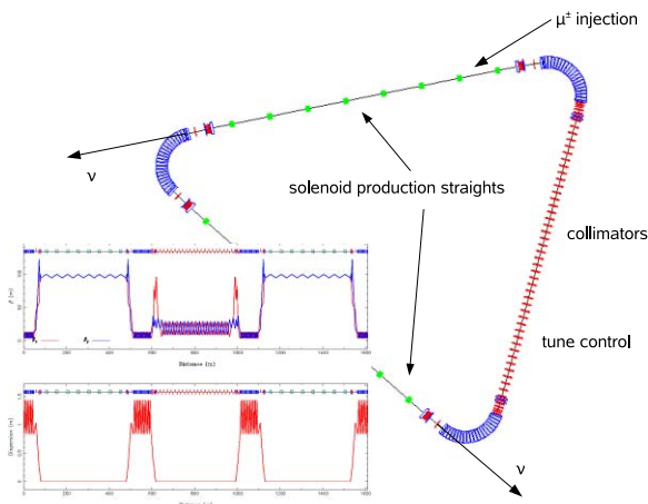
Figure 7: Isosceles decay ring, apex angle 52.8^\circ
