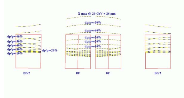
Figure 2: Magnets and orbit offsets in the “arc” cell.
