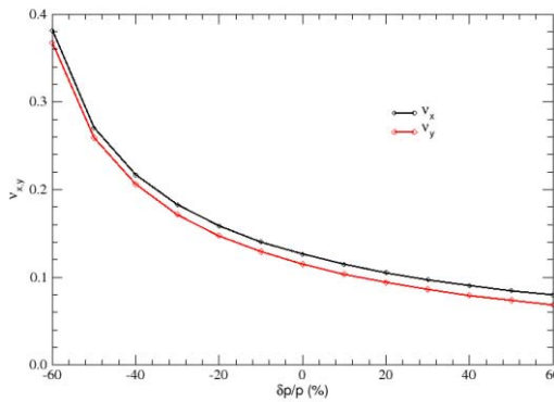
Figure 6: Betatron tunes versus momentum in the “IR” cell.
