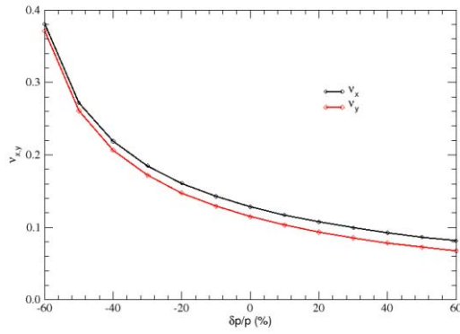
Figure 5: Betatron tunes versus momentum in the “arc” cell.
