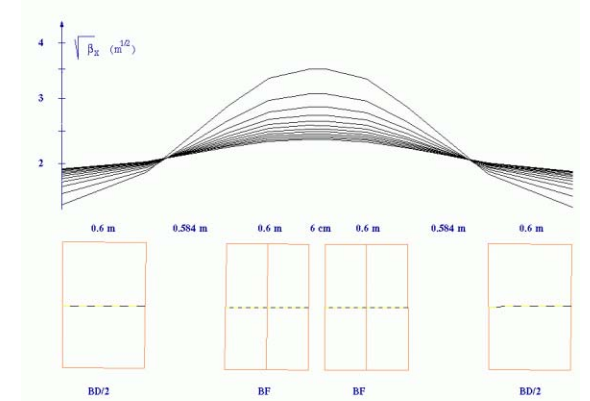
Figure 3: The horizontal betatron function in the “arc” cell.
