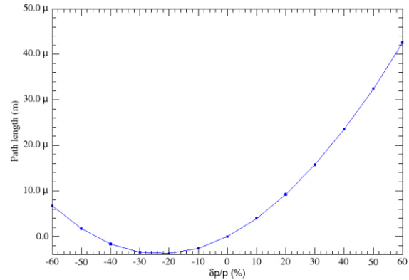
Figure 8: Path length dependence on momentum in the “IR” cell. (40μs corresponds to 0.133 ps ).
