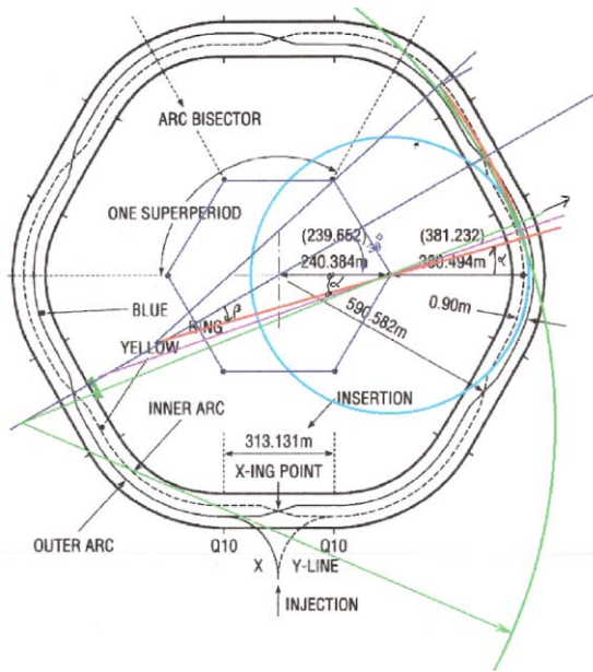
Figure 1: RHIC geometry with additional NS-FFAG arcs: one in the arc region presented by a part of the “magenta” circle and the other green colored within the IR region.
